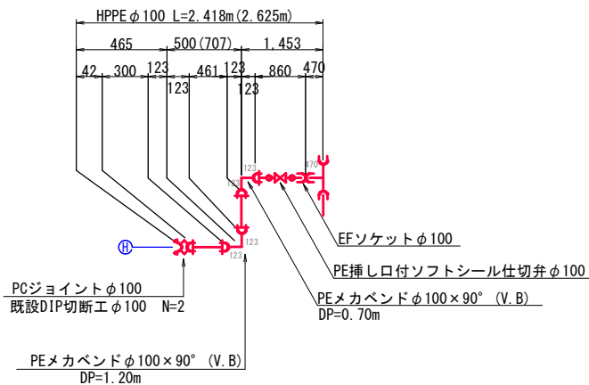
消火栓設置工 (1) No. 17+23.700
